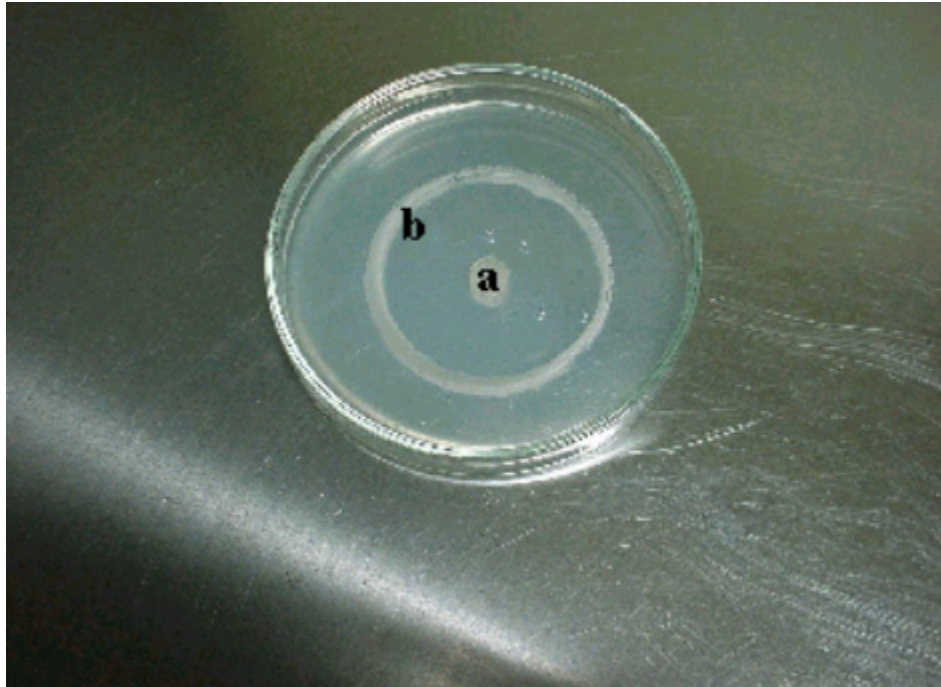
Figure 1. Dual cultures.
